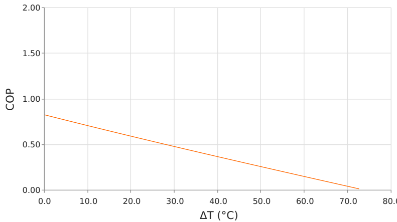
Coefficient of Performance (COP = Q_c/P_{in} ) T_{hot} = 35\text{ }^{\circ}\text{C} | I_{operating} = 5.6\text{ Amps}
