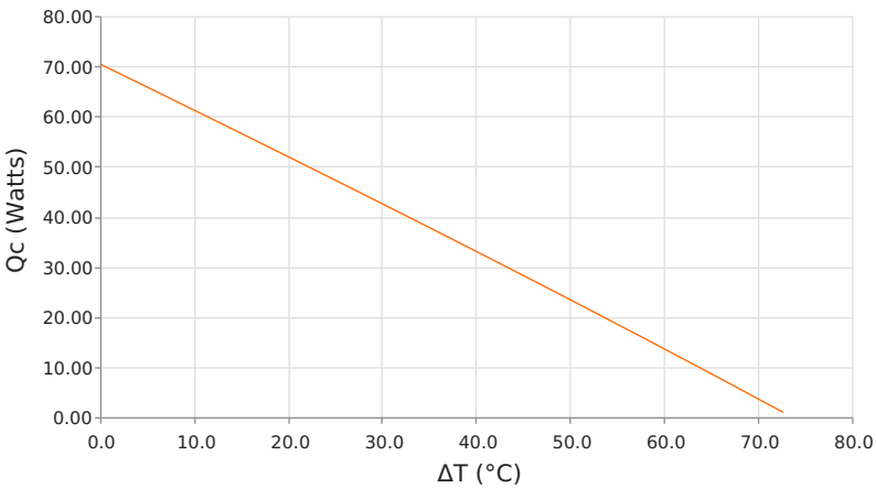
Heat Pumped at Cold Side ( Q_c ) T_{hot} = 35\text{ }^{\circ}\text{C} | I_{operating} = 5.6\text{ Amps}
