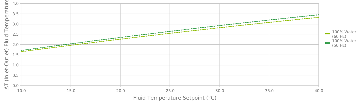
VRC2400-A1-20-BV2 \Delta T (Inlet-Outlet) Fluid Temperature Max System Cooling at 20°C Ambient Air 17.4 L/min Fluid Flow
