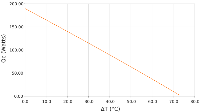
Heat Pumped at Cold Side ( Q_c ) T_{hot} = 35\text{ }^{\circ}\text{C} | operating = 8.4 Amps
