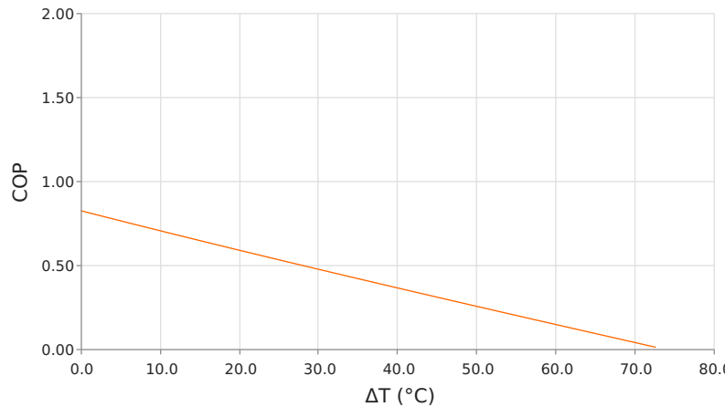
Coefficient of Performance (COP = Q_c/P_{in} ) T_{hot} = 35\text{ }^{\circ}\text{C} | operating = 8.4 Amps
