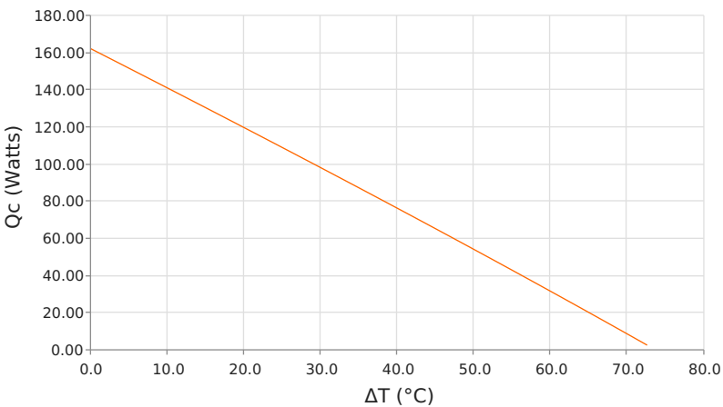
Heat Pumped at Cold Side (Qc) Thot = 35 °C | Ioperating = 7.2 Amps
