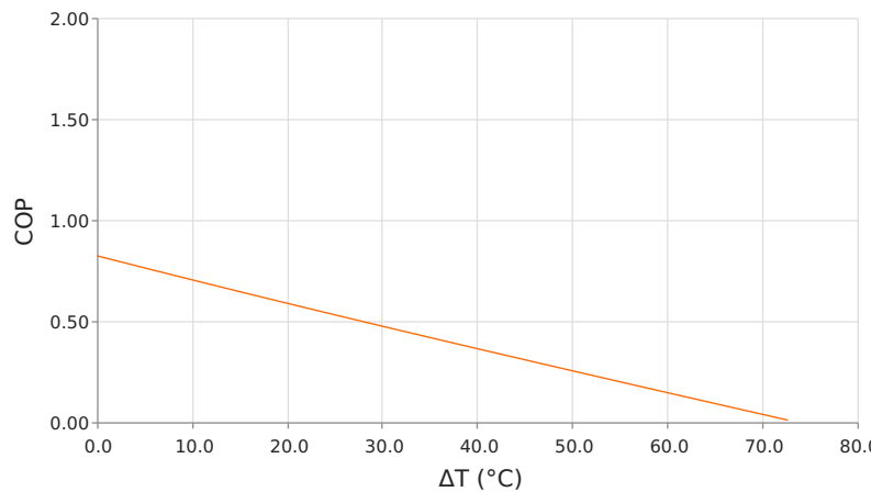
Coefficient of Performance (COP = Qc/Pin) Thot = 35 °C | Ioperating = 7.2 Amps
