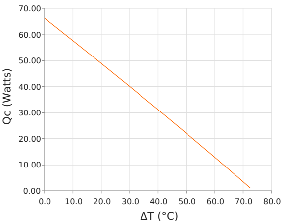
Heat Pumped at Cold Side ( Q_c ) T_{hot} = 35\text{ }^{\circ}\text{C} | operating = 6.7 Amps
