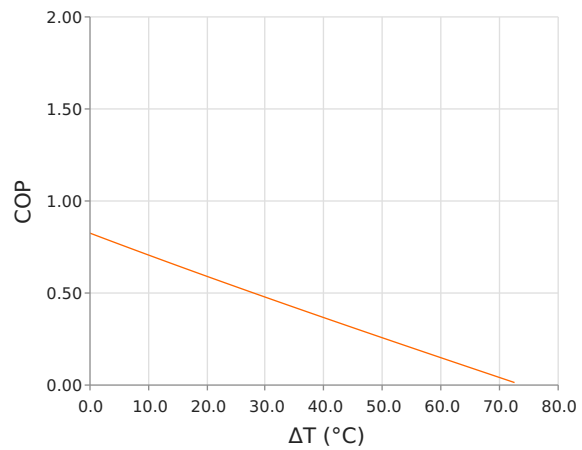
Coefficient of Performance (COP = Q_c/P_{in} ) T_{hot} = 35\text{ }^{\circ}\text{C} | operating = 6.7 Amps
