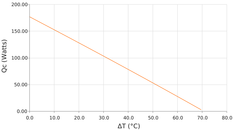
Heat Pumped at Cold Side ( Q_c ) T_{hot} = 35\text{ }^{\circ}\text{C} | I_{operating} = 8.4\text{ Amps}
