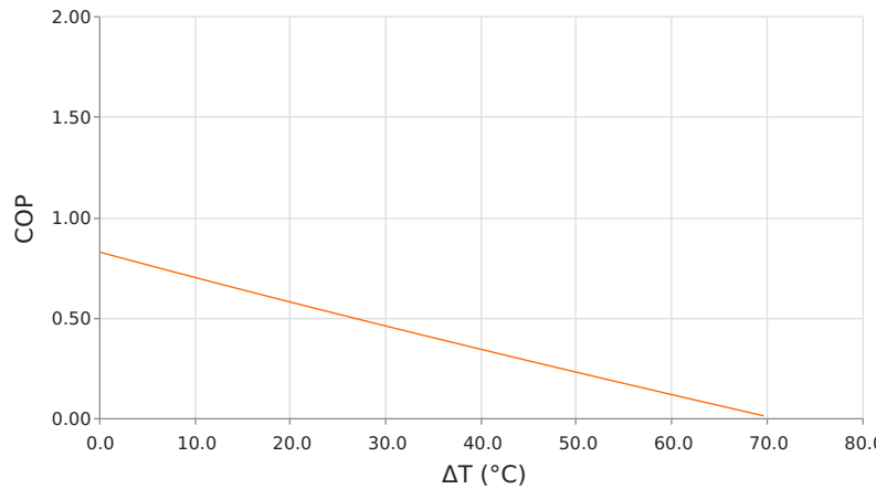
Coefficient of Performance (COP = Q_c/P_{in} ) T_{hot} = 35\text{ }^{\circ}\text{C} | I_{operating} = 8.4\text{ Amps}
