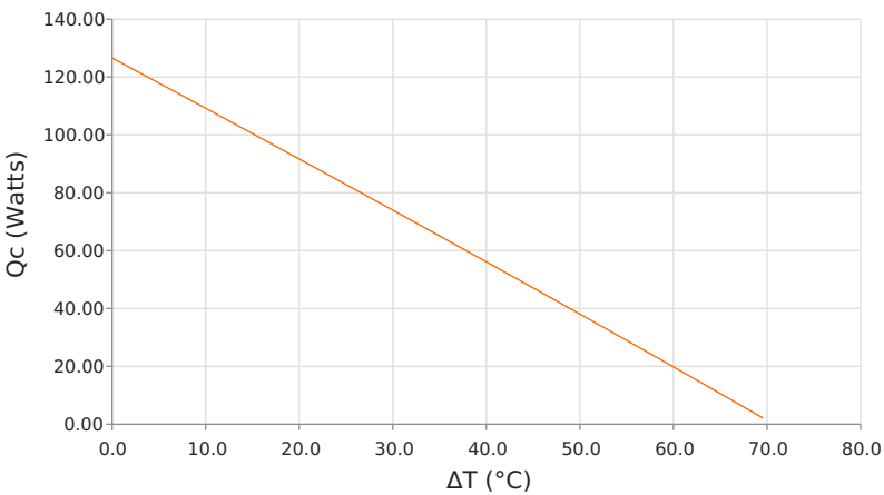
Heat Pumped at Cold Side ( Q_c ) T_{hot} = 35\text{ }^{\circ}\text{C} | Ioperating = 7.2 Amps
