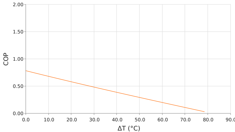
Coefficient of Performance (COP = Q_c/P_{in} ) T_{hot} = 50^\circ\text{C} | operating = 7.4 Amps
