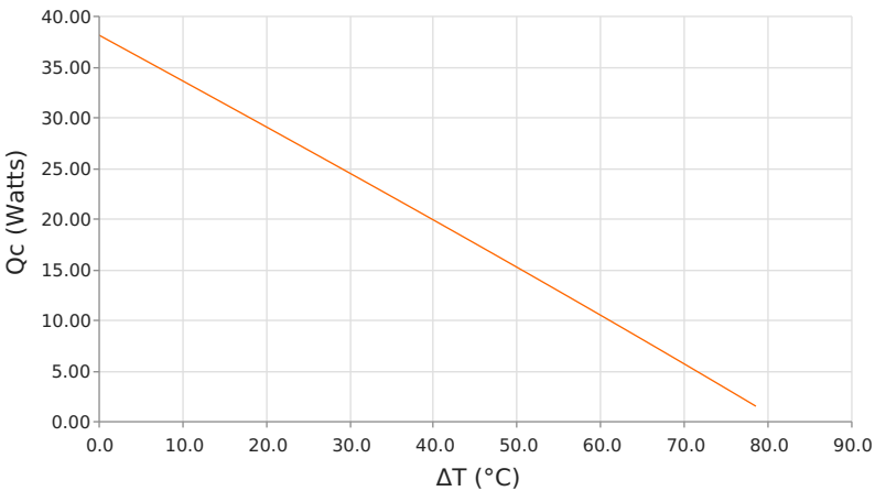
Heat Pumped at Cold Side ( Q_c ) T_{hot} = 50^\circ\text{C} | operating = 7.4 Amps
