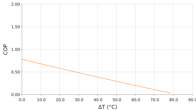
Coefficient of Performance (COP = Q_c/P_{in} ) T_{hot} = 50^\circ\text{C} | operating = 6.8 Amps
