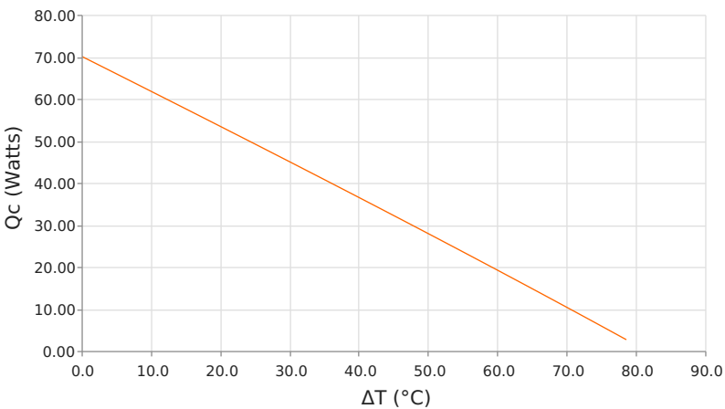
Heat Pumped at Cold Side ( Q_c ) T_{hot} = 50^\circ\text{C} | operating = 6.8 Amps
