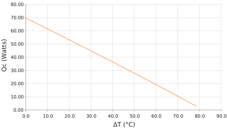
Heat Pumped at Cold Side ( Q_c ) T_{hot} = 50^{\circ}C | operating = 6.5 Amps
