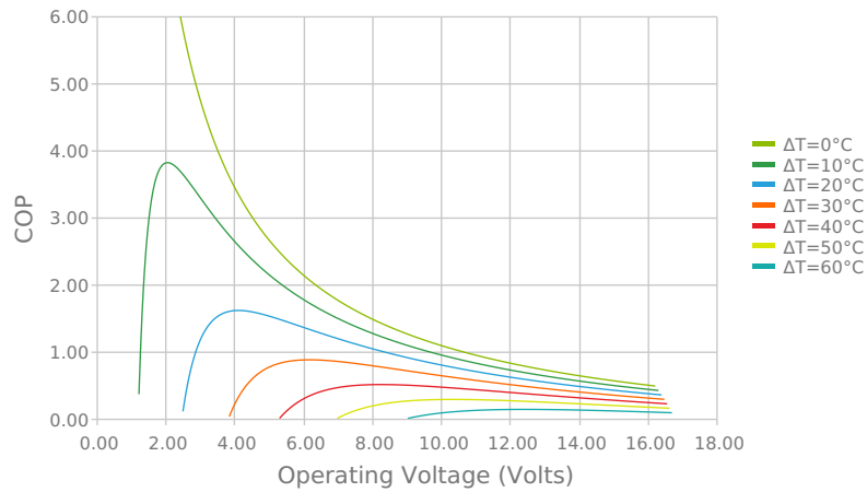
Coefficient of Performance ( COP = Q_c/P_{in} ) T_{hot} = 27^{\circ}C
