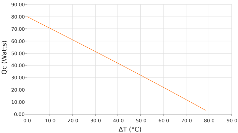
Heat Pumped at Cold Side ( Q_c ) T_{hot} = 50\text{ }^{\circ}\text{C} | operating = 6.2 Amps
