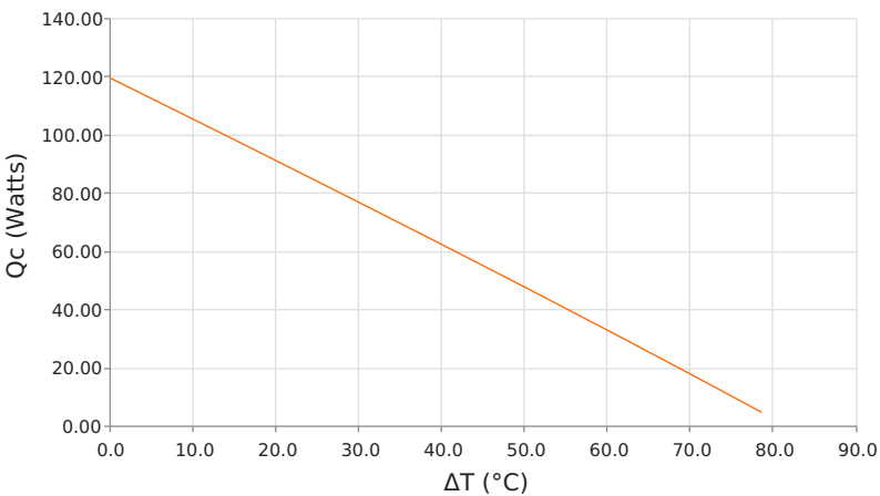
Heat Pumped at Cold Side ( Q_c ) T_{hot} = 50\text{ }^{\circ}\text{C} | operating = 5.1 Amps
