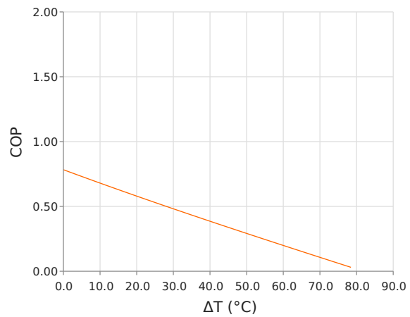
Coefficient of Performance (COP = Q_c/P_{in} ) T_{hot} = 50\text{ }^{\circ}\text{C} | operating = 3.4 Amps
