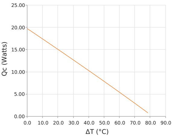
Heat Pumped at Cold Side ( Q_c ) T_{hot} = 50\text{ }^{\circ}\text{C} | operating = 3.4 Amps
