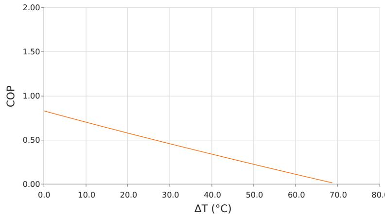
Coefficient of Performance (COP = Q_c/P_{in} ) T_{hot} = 35\text{ }^{\circ}\text{C} | I_{operating} = 1.3\text{ Amps}
