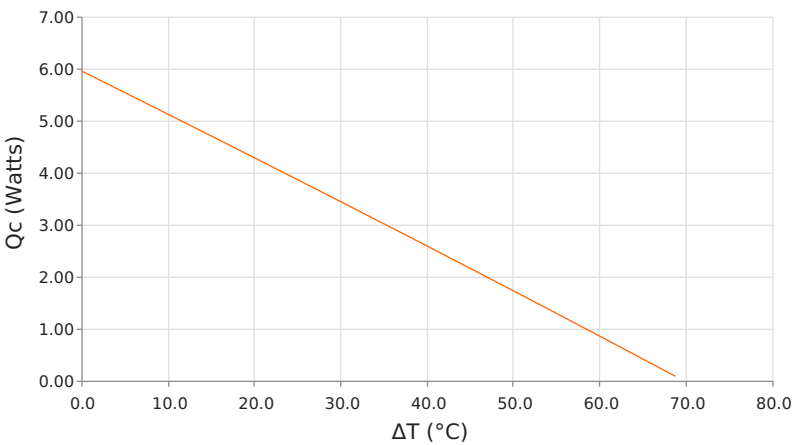
Heat Pumped at Cold Side ( Q_c ) T_{hot} = 35\text{ }^{\circ}\text{C} | I_{operating} = 1.3\text{ Amps}
