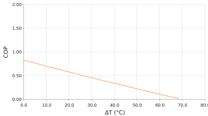
Coefficient of Performance (COP = Q_c/P_{in} ) T_{hot} = 35^\circ\text{C} | I_{operating} = 1\text{ Amps}
