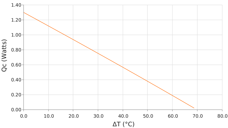
Heat Pumped at Cold Side ( Q_c ) T_{hot} = 35^\circ\text{C} | I_{operating} = 1\text{ Amps}
