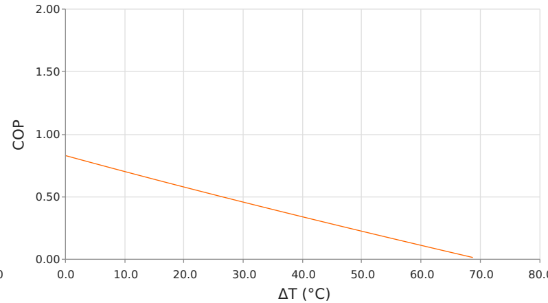
Coefficient of Performance (COP = Qc/Pin) Thot = 35 °C | Ioperating = 0.7 Amps
