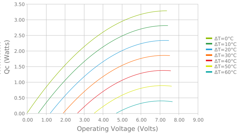
Heat Pumped at Cold Side Thot = 27 °C
