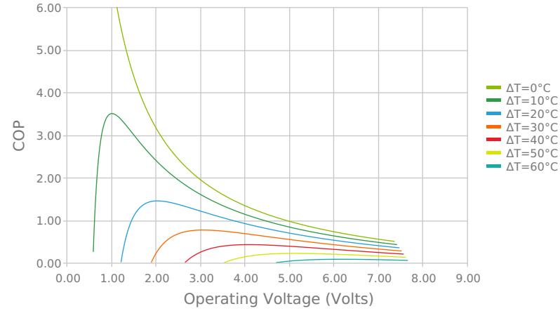
Coefficient of Performance (COP = Qc/Pin) Thot = 27 °C
