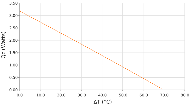
Heat Pumped at Cold Side (Qc) Thot = 35 °C | Ioperating = 0.7 Amps
