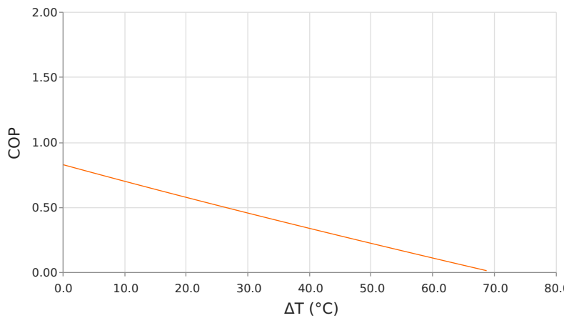
Coefficient of Performance (COP = Q_c/P_{in} ) T_{hot} = 35\text{ }^{\circ}\text{C} | I_{operating} = 0.7\text{ Amps}
