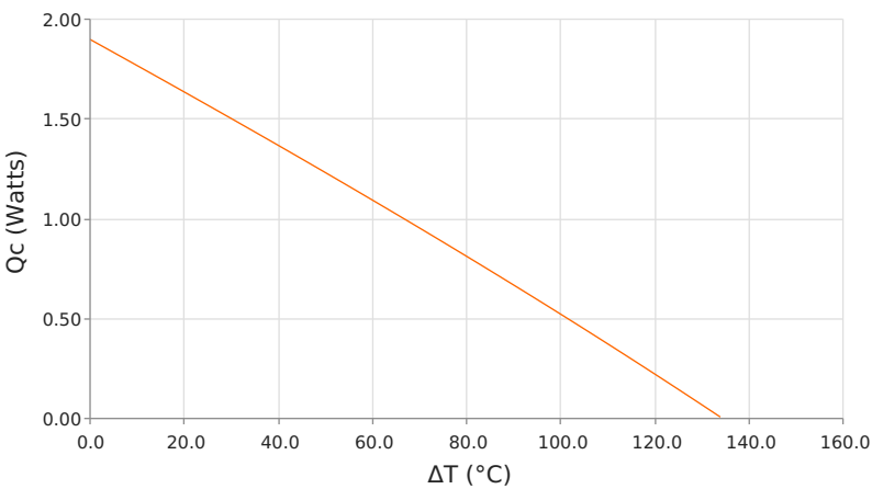
Heat Pumped at Cold Side ( Q_c ) T_{hot} = 35^\circ\text{C} | operating = 1.4 Amps
