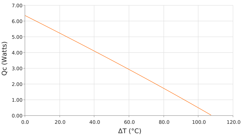
Heat Pumped at Cold Side ( Q_c ) T_{hot} = 35\text{ }^{\circ}\text{C} | operating = 1.6 Amps
