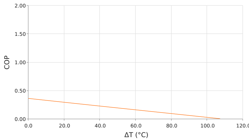
Coefficient of Performance (COP = Q_c/P_{in} ) T_{hot} = 35\text{ }^{\circ}\text{C} | operating = 1.6 Amps
