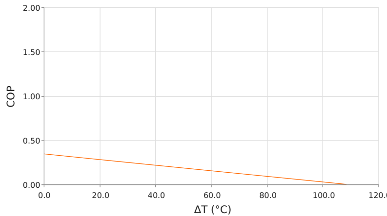
Coefficient of Performance (COP = Q_c/P_{in} ) T_{hot} = 35\text{ }^{\circ}\text{C} | operating = 3.1 Amps
