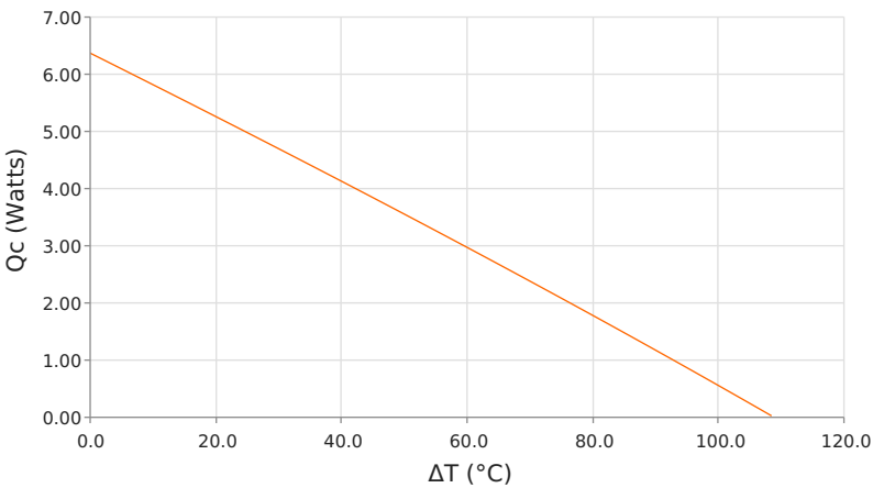
Heat Pumped at Cold Side ( Q_c ) T_{hot} = 35\text{ }^{\circ}\text{C} | operating = 3.1 Amps
