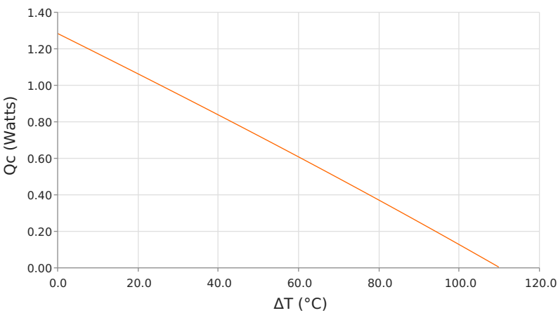
Heat Pumped at Cold Side ( Q_c ) T_{hot} = 35\text{ }^{\circ}\text{C} | operating = 1.5 Amps
