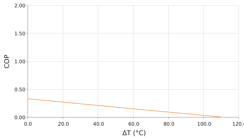
Coefficient of Performance (COP = Q_c/P_{in} ) T_{hot} = 35\text{ }^{\circ}\text{C} | operating = 1.5 Amps
