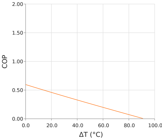
Coefficient of Performance (COP = Q_c/P_{in} ) Thot = 35 °C | Ioperating = 3.9 Amps
