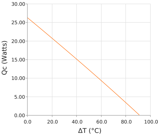
Heat Pumped at Cold Side ( Q_c ) Thot = 35 °C | Ioperating = 3.9 Amps
