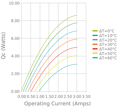
Heat Pumped at Cold Side Thot = 27 °C
