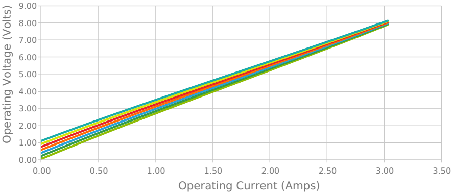
Current vs Voltage (I vs V) Thot = 27 °C
