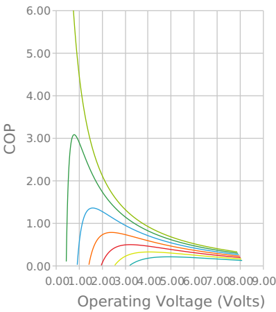
Coefficient of Performance (COP = Q_c/P_{in} ) T_{hot} = 27\text{ }^{\circ}\text{C}
