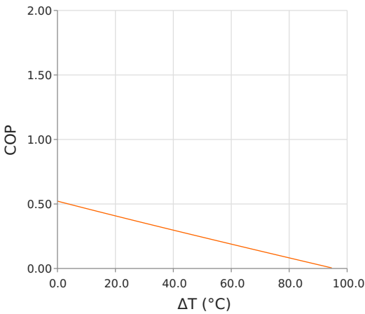
Coefficient of Performance (COP = Q_c/P_{in} ) T_{hot} = 35\text{ }^{\circ}\text{C} | I_{operating} = 3.4\text{ Amps}
