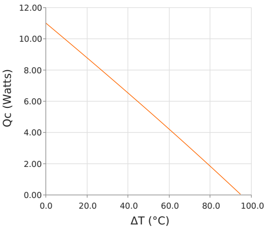
Heat Pumped at Cold Side ( Q_c ) T_{hot} = 35\text{ }^{\circ}\text{C} | I_{operating} = 3.4\text{ Amps}
