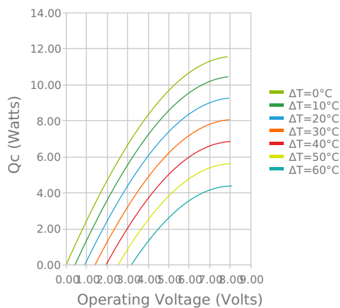
Heat Pumped at Cold Side T_{hot} = 27^\circ \text{C}
