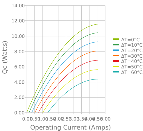
Heat Pumped at Cold Side T_{hot} = 27^\circ\text{C}
