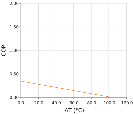
Coefficient of Performance (COP = Q_c/P_{in} ) Thot = 35 °C | Ioperating = 0.7 Amps
