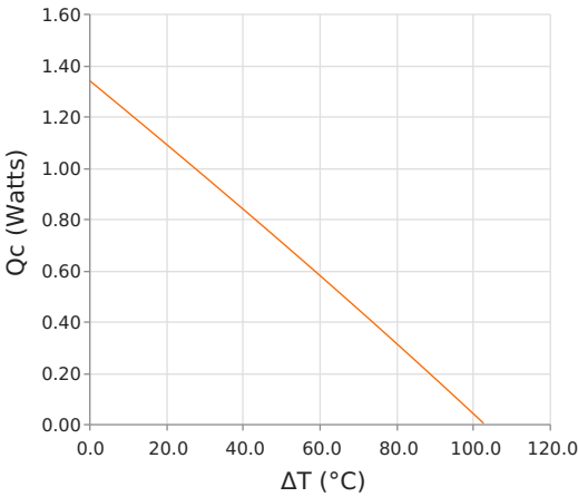
Heat Pumped at Cold Side ( Q_c ) Thot = 35 °C | Ioperating = 0.7 Amps
