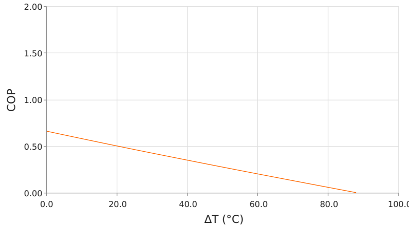
Coefficient of Performance (COP = Q_c/P_{in} ) T_{hot} = 35\text{ }^{\circ}\text{C} | operating = 0.4 Amps
