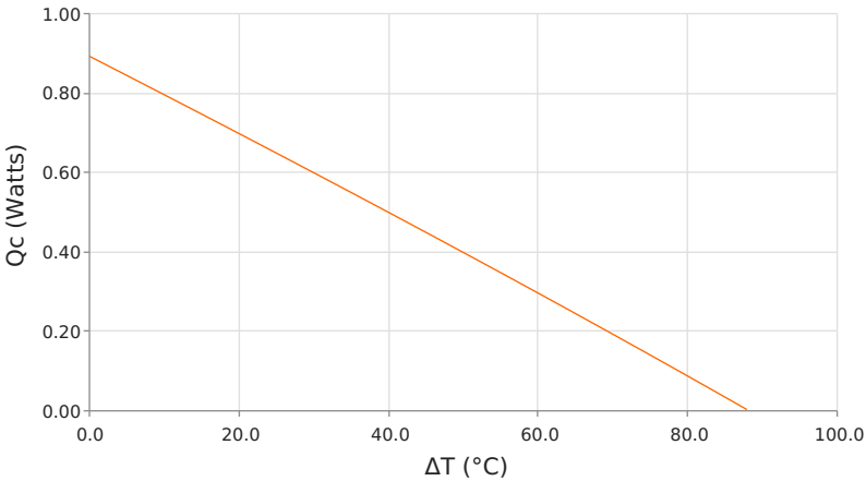
Heat Pumped at Cold Side ( Q_c ) T_{hot} = 35\text{ }^{\circ}\text{C} | operating = 0.4 Amps
