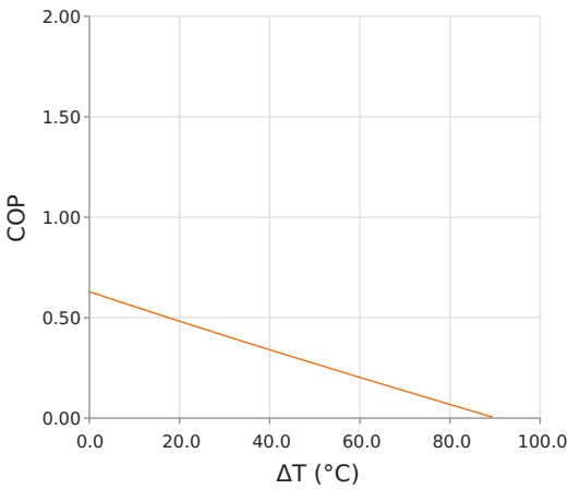
Coefficient of Performance (COP = Q_c/P_{in} ) Thot = 35 °C | Ioperating = 3.5 Amps
