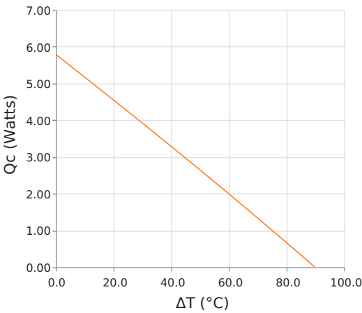
Heat Pumped at Cold Side ( Q_c ) Thot = 35 °C | Ioperating = 3.5 Amps
