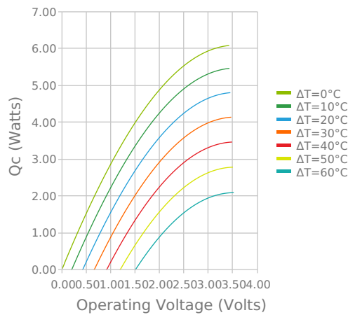
Heat Pumped at Cold Side Thot = 27 °C
