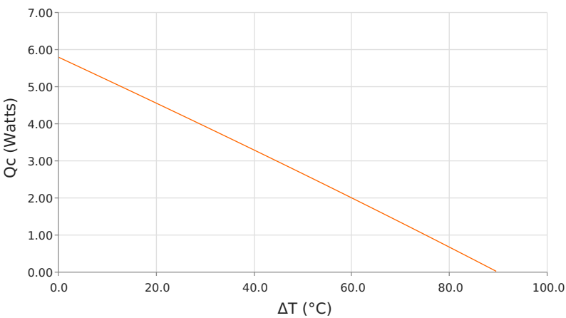
Heat Pumped at Cold Side ( Q_c ) T_{hot} = 35^\circ\text{C} | operating = 3.5 Amps
