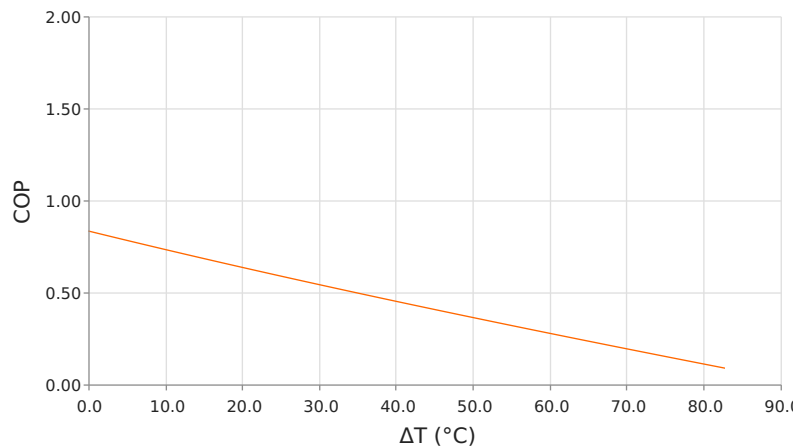
Coefficient of Performance (COP = Q_c/P_{in} ) T_{hot} = 85\text{ }^{\circ}\text{C} | operating = 7 Amps
