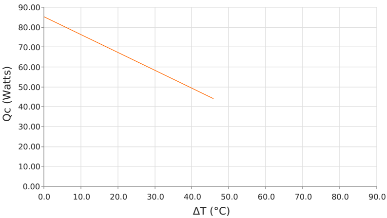
Heat Pumped at Cold Side ( Q_c ) T_{hot} = 85^\circ\text{C} | operating = 7 Amps
