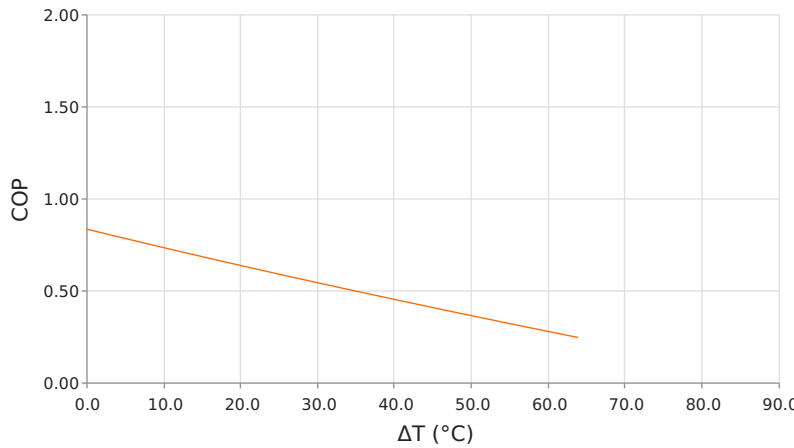
Coefficient of Performance (COP = Q_c/P_{in} ) T_{hot} = 85^\circ\text{C} | operating = 7 Amps
