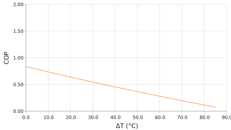
Coefficient of Performance (COP = Q_c/P_{in} ) T_{hot} = 85^\circ\text{C} | operating = 6.3 Amps
