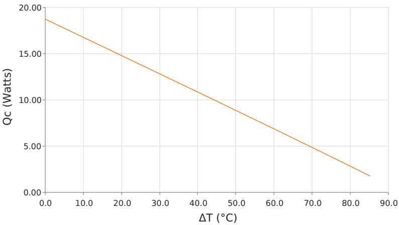
Heat Pumped at Cold Side ( Q_c ) T_{hot} = 85^\circ\text{C} | operating = 6.3 Amps
