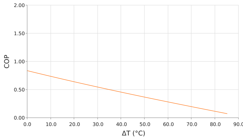
Coefficient of Performance (COP = Q_c/P_{in} ) T_{hot} = 85\text{ }^{\circ}\text{C} | operating = 5.5 Amps
