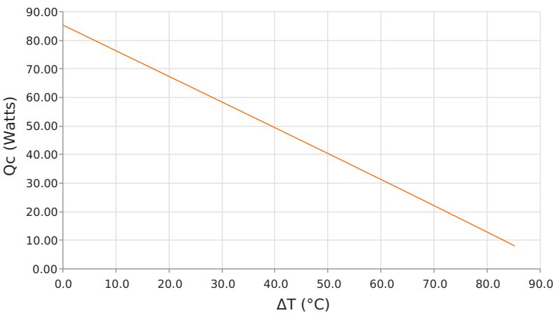
Heat Pumped at Cold Side ( Q_c ) T_{hot} = 85\text{ }^{\circ}\text{C} | operating = 5.5 Amps
