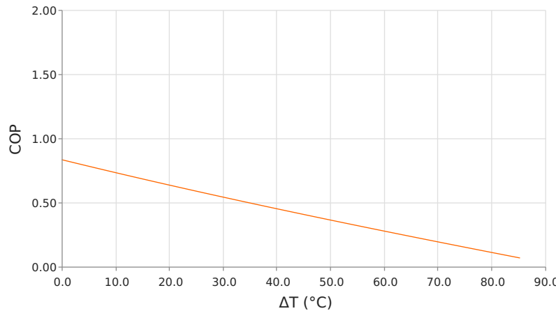
Coefficient of Performance (COP = Q_c/P_{in} ) T_{hot} = 85^\circ\text{C} | operating = 2 Amps
