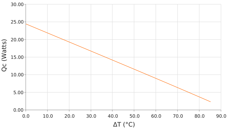
Heat Pumped at Cold Side ( Q_c ) T_{hot} = 85^\circ\text{C} | operating = 2 Amps
