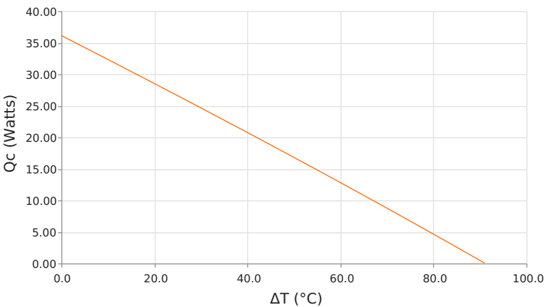
Heat Pumped at Cold Side ( Q_c ) T_{hot} = 35^\circ\text{C} | operating = 5.4 Amps
