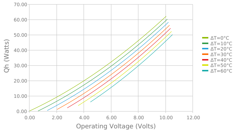
Total Heat Dissipated at Hot Side ( Q_h=Q_c+P_{in} ) T_{hot} = 85^\circ\text{C}
