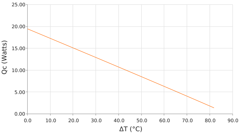
Heat Pumped at Cold Side ( Q_c ) T_{hot} = 85^\circ\text{C} | I_{operating} = 3.1 Amps
