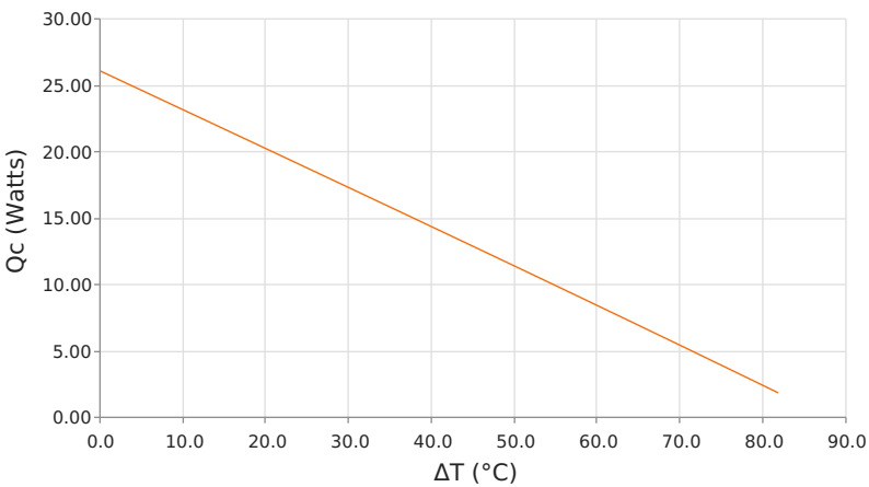
Heat Pumped at Cold Side ( Q_c ) T_{hot} = 85\text{ }^{\circ}\text{C} | operating = 2.3 Amps
