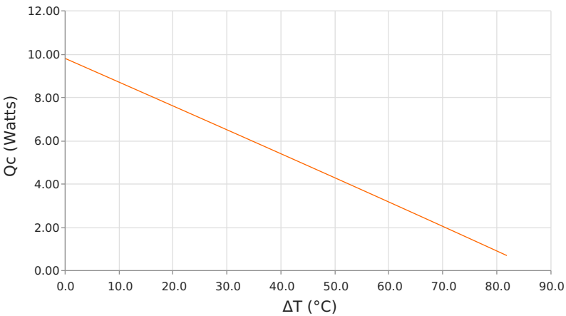
Heat Pumped at Cold Side ( Q_c ) T_{hot} = 85\text{ }^{\circ}\text{C} | operating = 1.6 Amps
