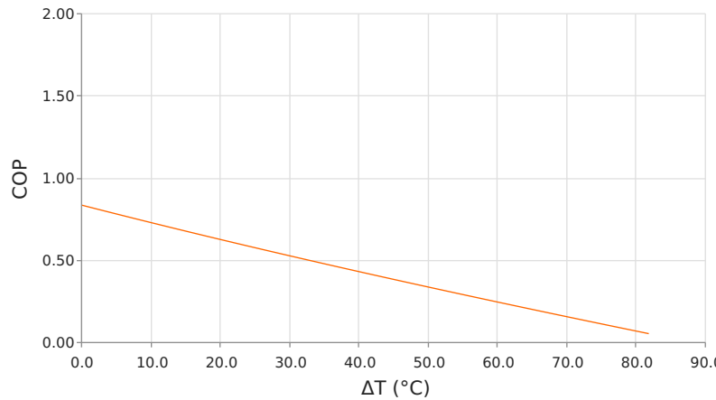
Coefficient of Performance (COP = Q_c/P_{in} ) T_{hot} = 85\text{ }^{\circ}\text{C} | operating = 1.6 Amps
