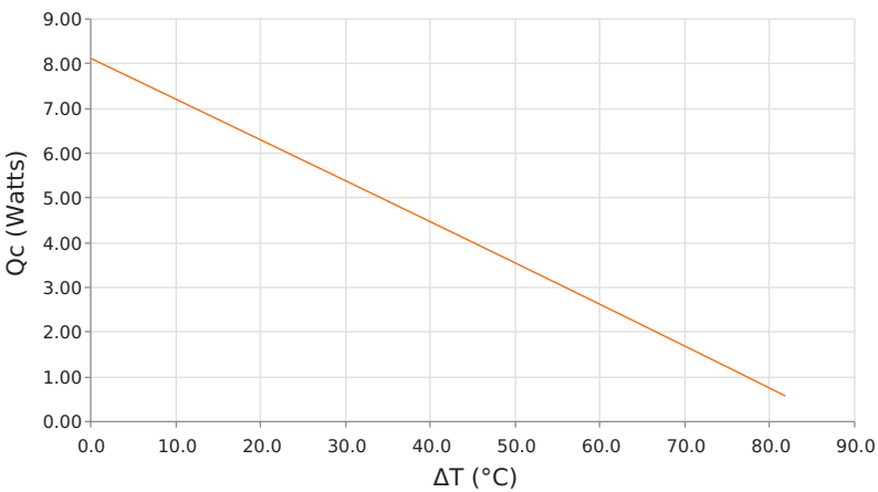
Heat Pumped at Cold Side ( Q_c ) T_{hot} = 85\text{ }^{\circ}\text{C} | operating = 1.9 Amps
