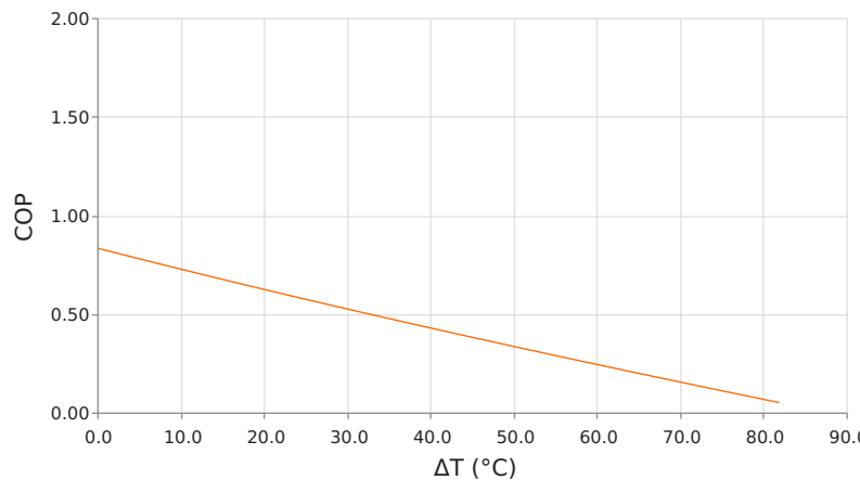
Coefficient of Performance (COP = Q_c/P_{in} ) T_{hot} = 85\text{ }^{\circ}\text{C} | I_{operating} = 2.1\text{ Amps}
