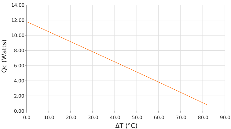
Heat Pumped at Cold Side ( Q_c ) T_{hot} = 85\text{ }^{\circ}\text{C} | I_{operating} = 2.1\text{ Amps}
