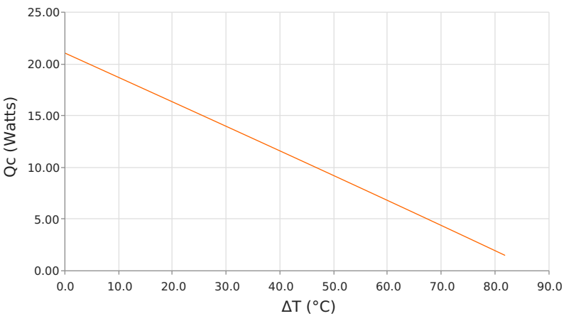
Heat Pumped at Cold Side ( Q_c ) T_{hot} = 85\text{ }^{\circ}\text{C} | I_{operating} = 1.9\text{ Amps}
