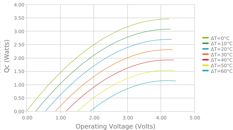
Heat Pumped at Cold Side T_{hot} = 85\text{ }^{\circ}\text{C}
