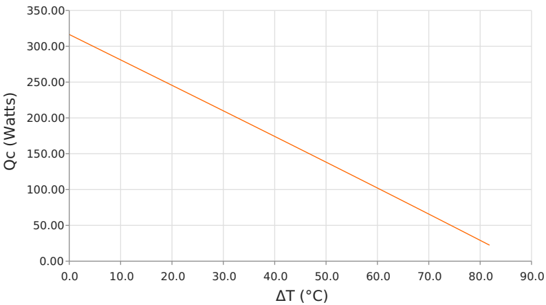
Heat Pumped at Cold Side ( Q_c ) T_{hot} = 85\text{ }^{\circ}\text{C} | I_{operating} = 12.4\text{ Amps}
