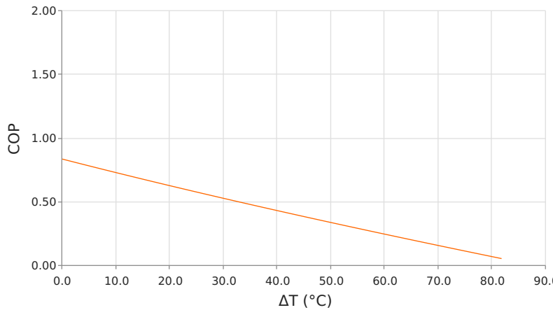
Coefficient of Performance (COP = Q_c/P_{in} ) T_{hot} = 85\text{ }^{\circ}\text{C} | I_{operating} = 12.4\text{ Amps}
