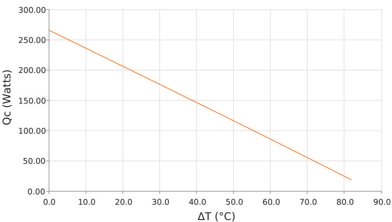
Heat Pumped at Cold Side ( Q_c ) T_{hot} = 85\text{ }^{\circ}\text{C} | operating = 12.4 Amps
