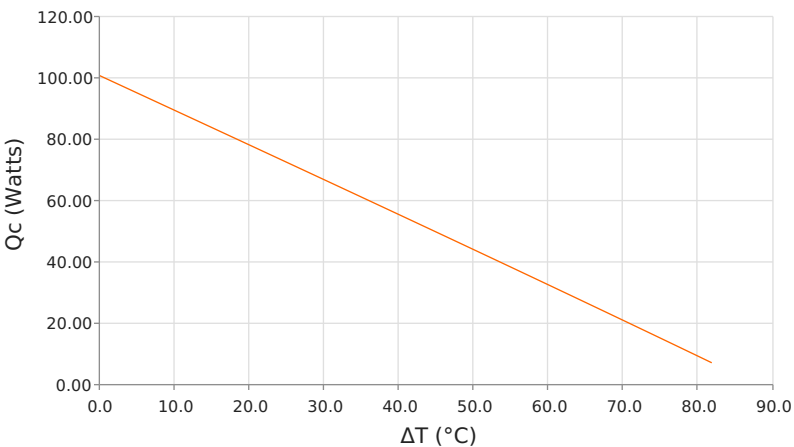
Heat Pumped at Cold Side ( Q_c ) T_{hot} = 85\text{ }^{\circ}\text{C} | operating = 9 Amps
