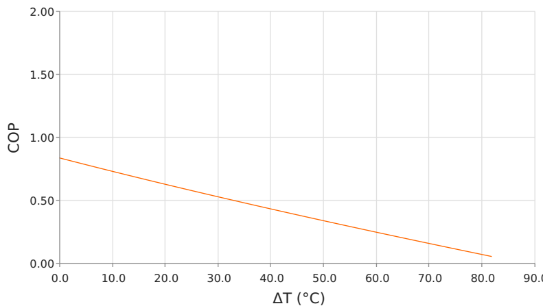
Coefficient of Performance (COP = Q_c/P_{in} ) T_{hot} = 85\text{ }^{\circ}\text{C} | operating = 9 Amps
