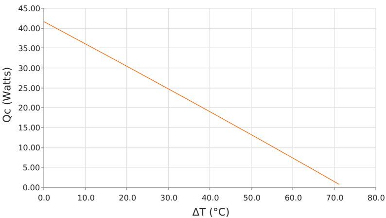
Heat Pumped at Cold Side ( Q_c ) T_{hot} = 35\text{ }^{\circ}\text{C} | operating = 7.9 Amps
