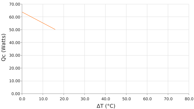
Heat Pumped at Cold Side ( Q_c ) T_{hot} = 35^\circ\text{C} | operating = 12.1 Amps
