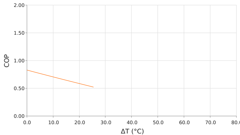
Coefficient of Performance (COP = Q_c/P_{in} ) T_{hot} = 35^\circ\text{C} | operating = 12.1 Amps
