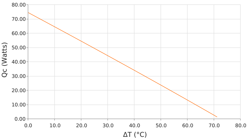
Heat Pumped at Cold Side (Qc) Thot = 35 °C | Ioperating = 7.9 Amps
